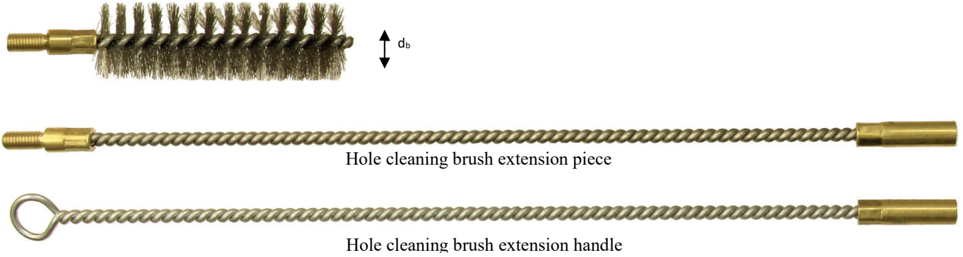
FIGURE 4 – HOLE CLEANING BRUSHES
